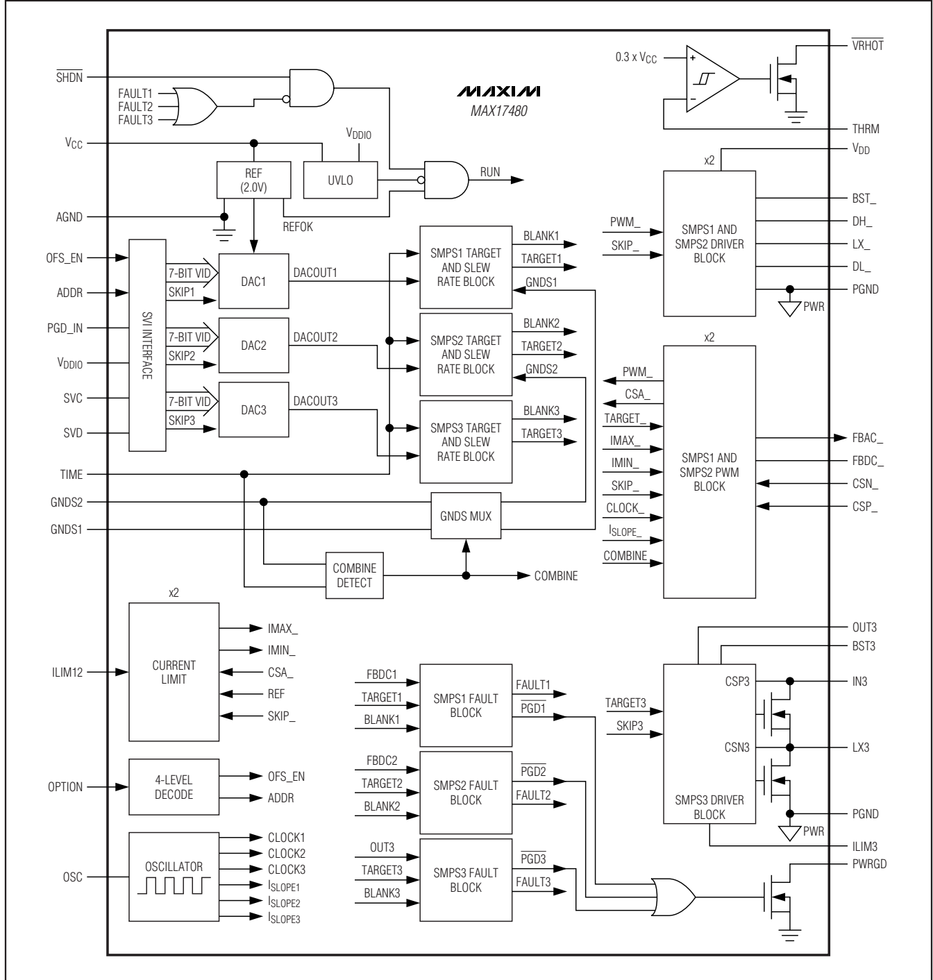
Figure 4. Functional Diagram
