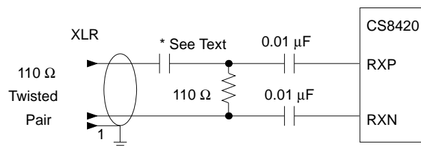
Figure 34. Transformerless Professional Input Circuit
