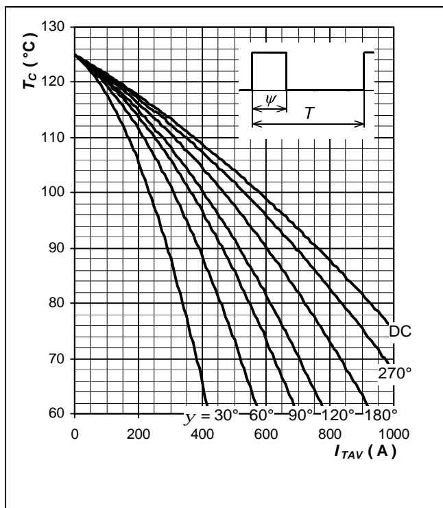
Fig. 9 Max. case temperature vs. average forward current, square waveform, f = 50 Hz, T = 1/f
