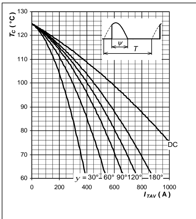
Fig. 8 Max. case temperature vs. average forward current, sine waveform, f = 50 Hz, T = 1/f
