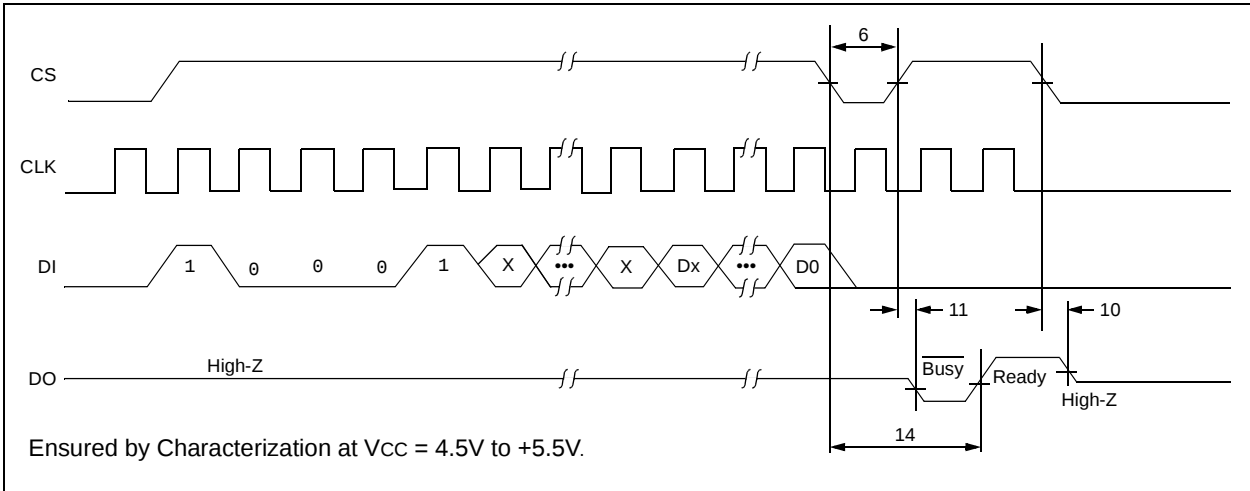
FIGURE 2-5: WRAL TIMING
