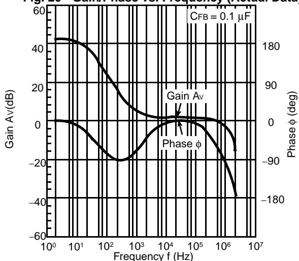
Fig. 20 - Gain/Phase vs. Frequency (Actual Data)
