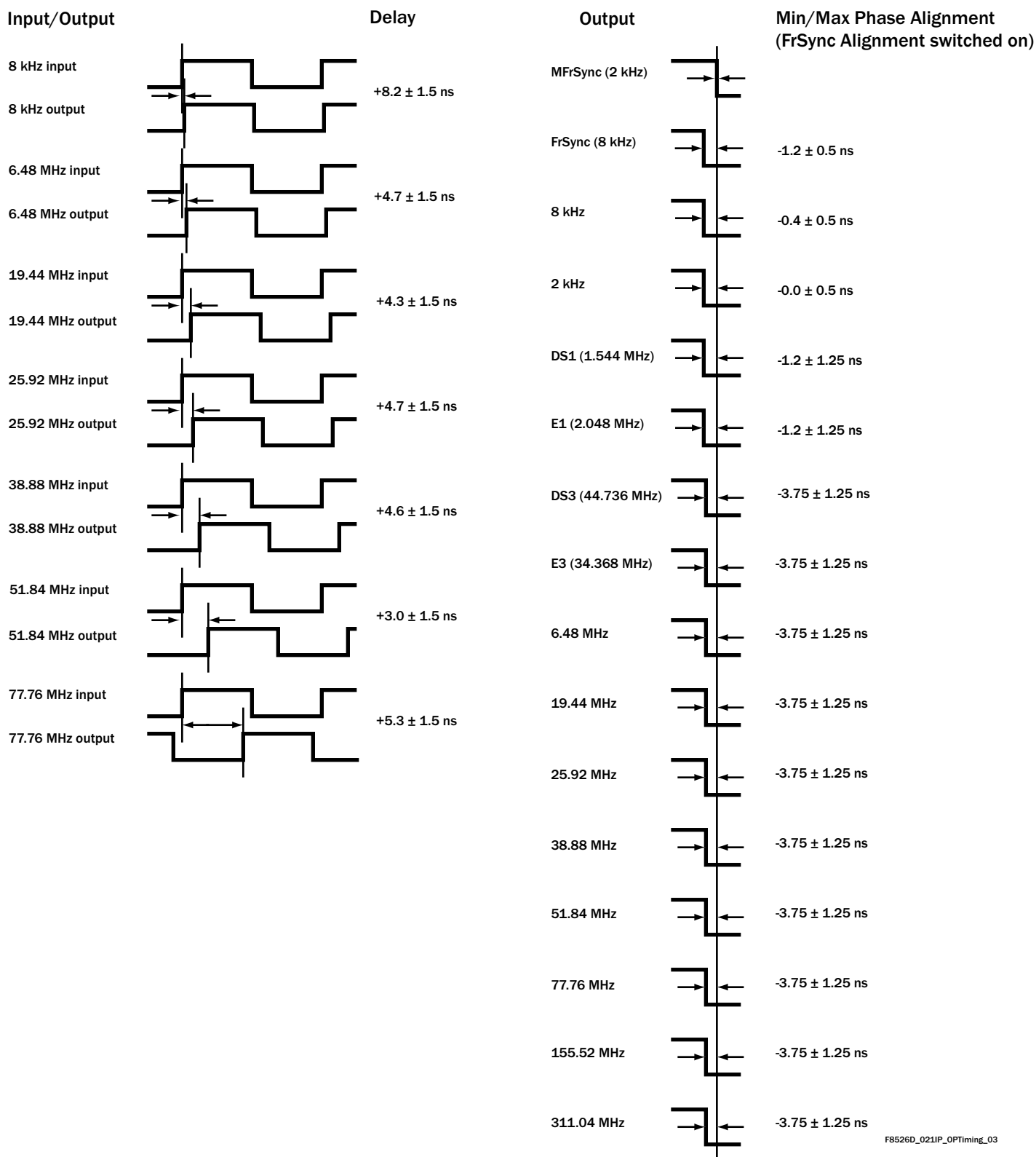
Figure 12 Input/Output Timing (Typical Conditions)
