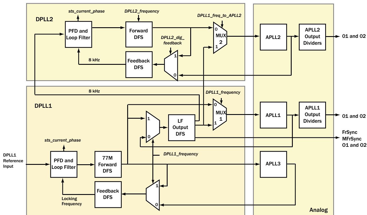
Figure 4 PLL Block Diagram
