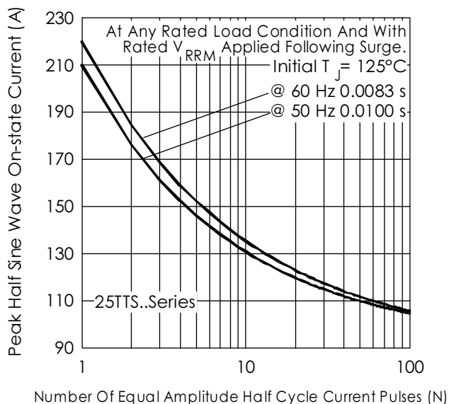
Fig. 6 - Maximum Non-Repetitive Surge Current
