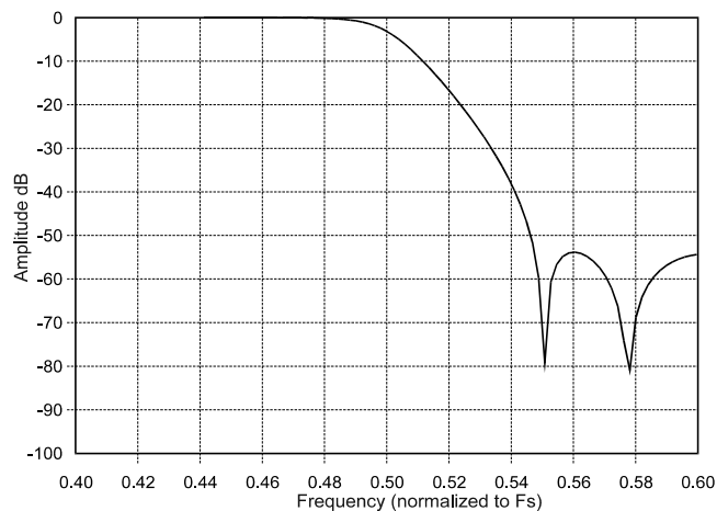
Figure 16. Transition Band
