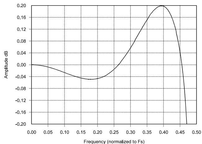
Figure 22. Passband Ripple
