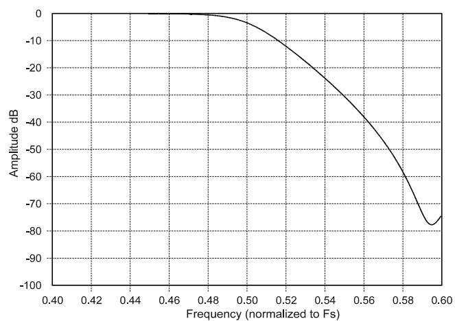
Figure 20. Transition Band
