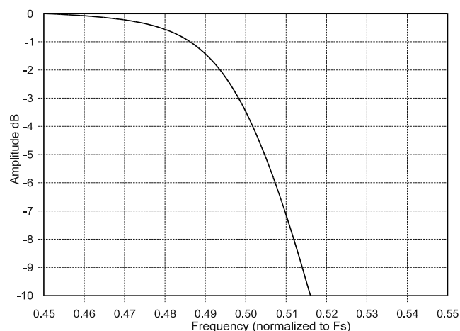
Figure 21. Transition Band
