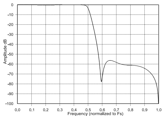
Figure 19. Stopband Rejection
