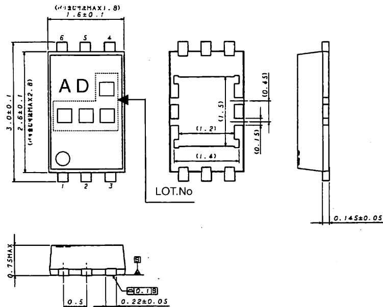
HVSO6-6 (Unit:mm)
