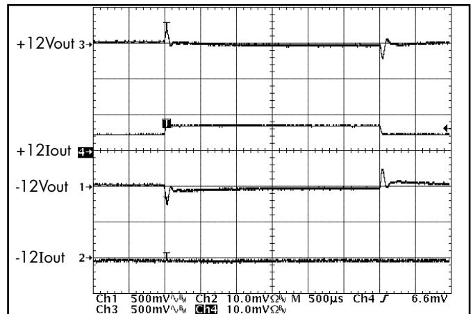
Figure 22: Output voltage response to step-change in I_{out2} (50%-75%-50% of I_{max} ; dI/dt = 0.1A/\mu s ). Load cap: 15 \mu F , 300 m \Omega ESR tantalum cap & 1 \mu F ceramic cap.. V_{out} (500mV/div), I_{out} (5A/div). Ch1: V_{out1} ; Ch2 I_{out2} ; Ch 3: V_{out2} ; Ch 4 I_{out2}
