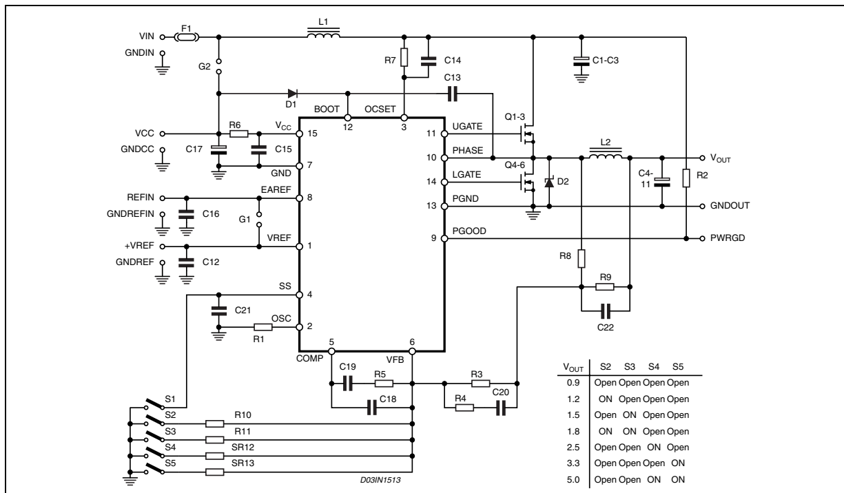
Figure 12. 15A Demo Board Schematic
