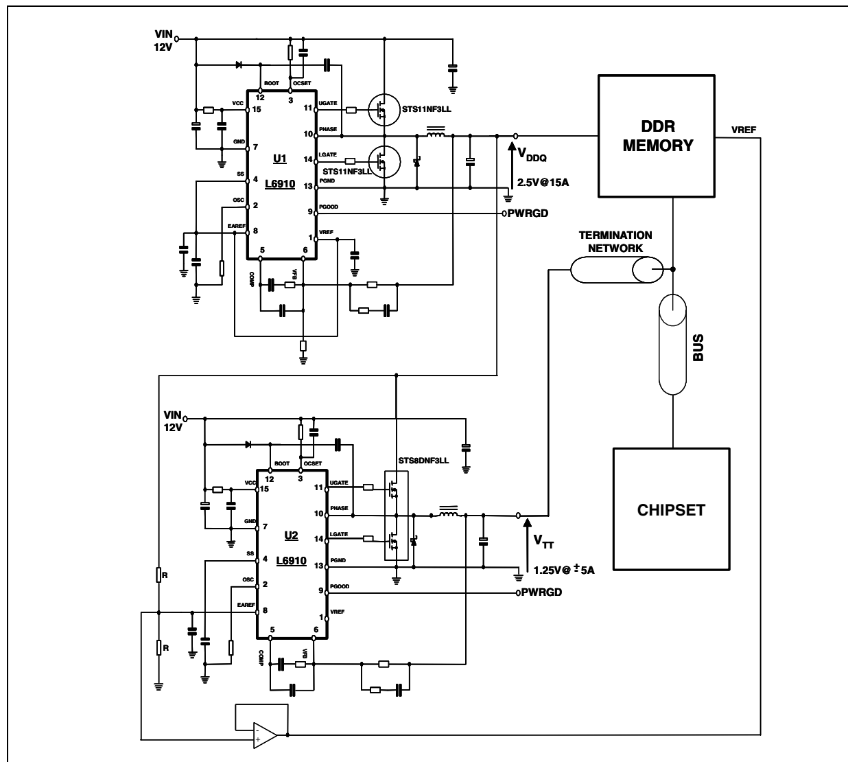
Figure 21. Application idea : DDR Memory Supply
