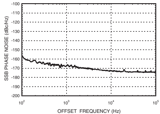
Phase Noise at Pout = 10 dBm @ 9 GHz
