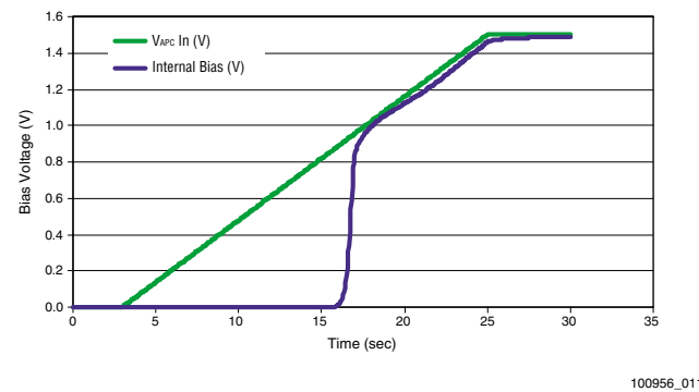
Figure 10. PAM Internal Bias Performance – No Pedestal Applied
