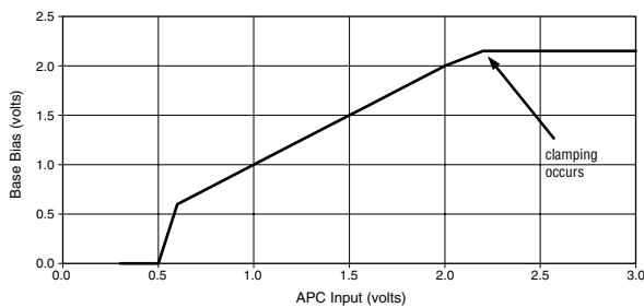
Figure 8. Base Bias Voltage vs. APC Input, V_{CC} = 4.0 V
