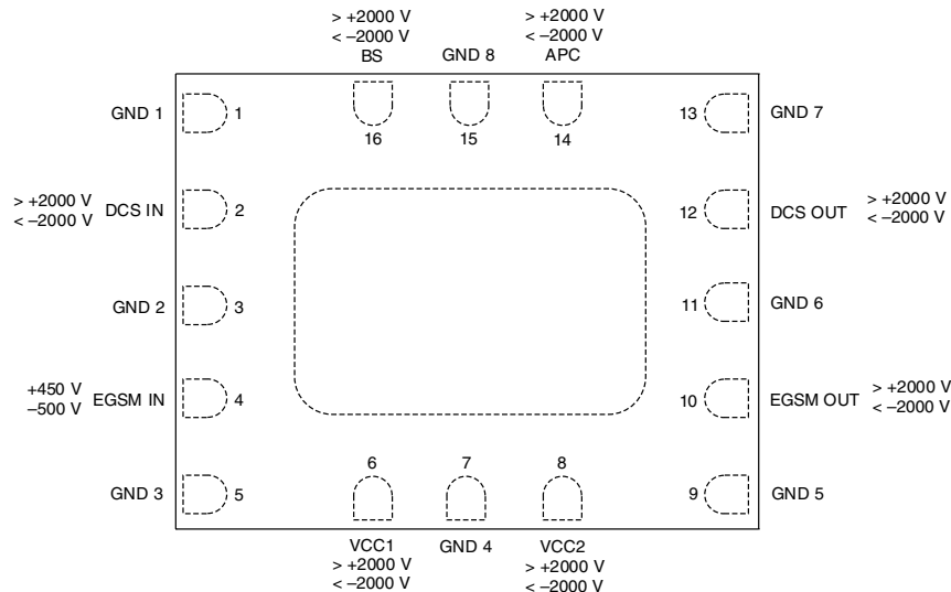
Figure 6. ESD Sensitivity Areas (Top View)
