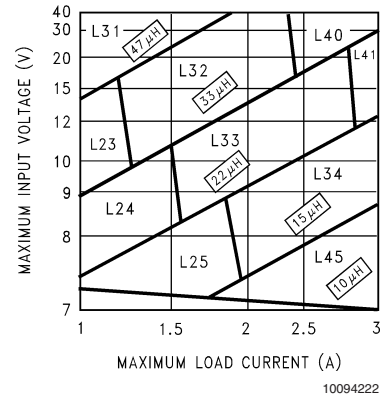
FIGURE 4. LM2670-5.0
