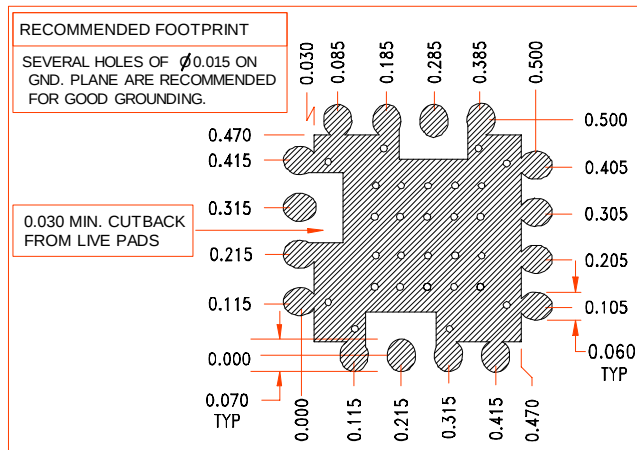
Footprint
