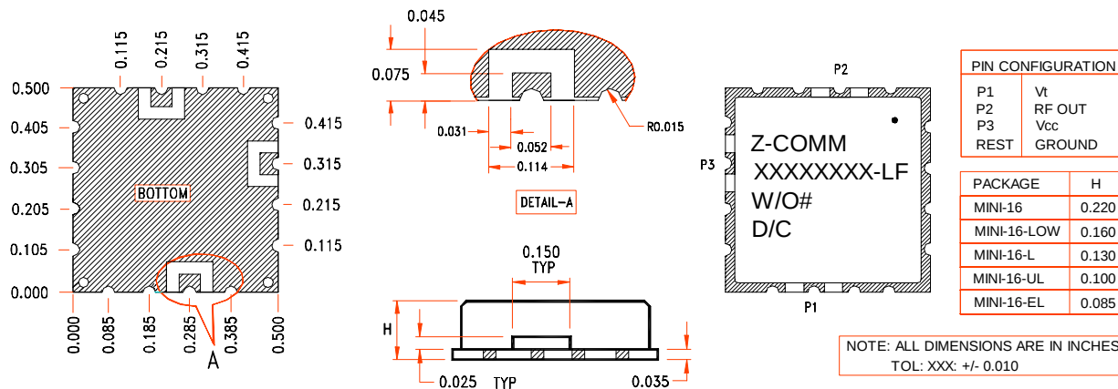
Physical Dimensions
