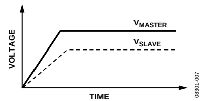
Figure 44. Ratiometric Tracking
