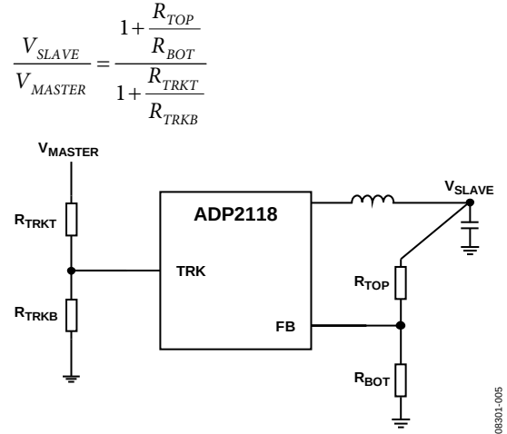
Figure 42. Voltage Tracking
