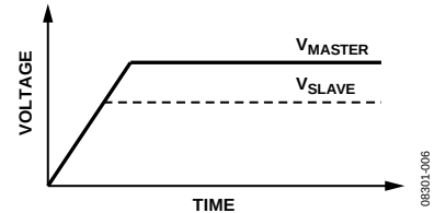
Figure 43. Coincident Tracking
