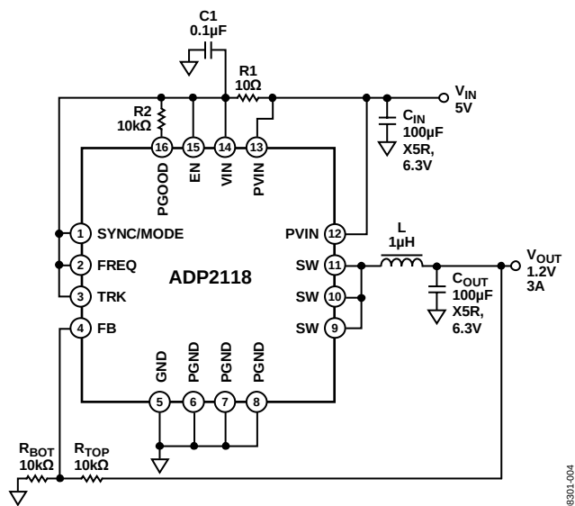
Figure 41. Application Circuit
