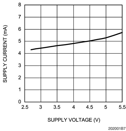
Supply Current vs Supply Voltage CC Headphone Mode, No Load
