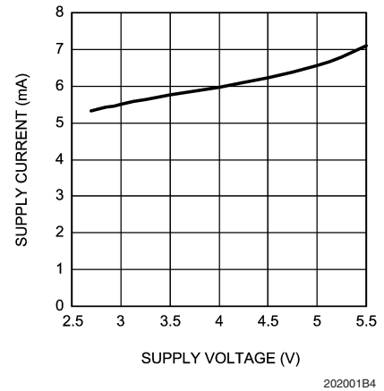
Supply Current vs Supply Voltage Speaker and OCL Headphone Mode, No Load
