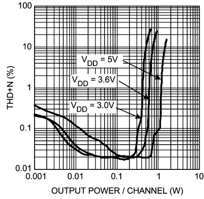
THD+N vs Output Power Speaker Mode, Differential Input A_V = 6\text{dB} , R_L = 8\Omega , f = 1\text{kHz}
