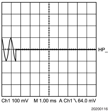
Turn-Off CC Headphone Mode
