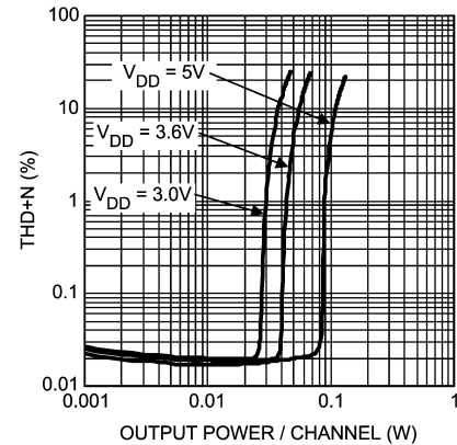
THD+N vs Output Power OCL Headphone Mode, Single-Ended Input A_V = 0\text{dB} , R_L = 32\Omega , f = 1\text{kHz}
