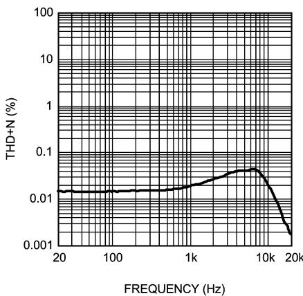
THD+N vs Frequency OCL Headphone Mode, Single-Ended Input V_{DD} = 3.6V , P_{OUT} = 30mW , R_L = 32\Omega
