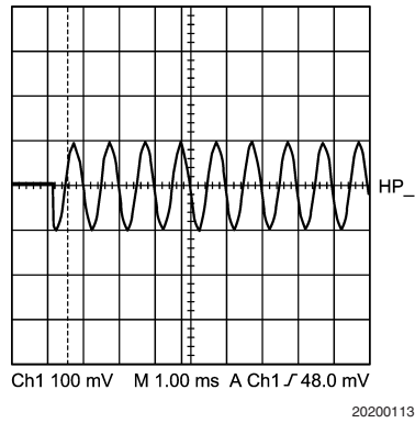
Turn-On OCL Headphone Mode
