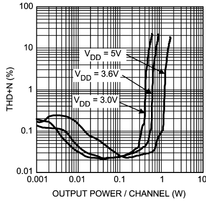
THD+N vs Output Power Speaker Mode, Single-Ended Input A_V = 6\text{dB} , R_L = 8\Omega , f = 1\text{kHz}
