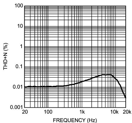
THD+N vs Frequency OCL Headphone Mode, Differential Input V_{DD} = 3.6V, P_{OUT} = 30mW, R_L = 32\Omega
