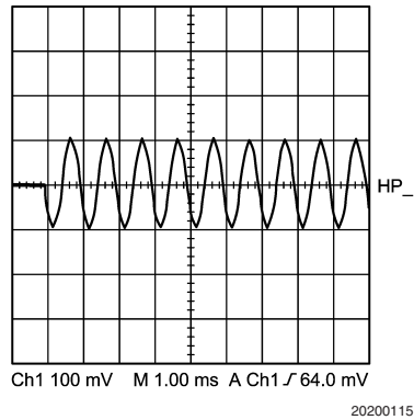
Turn-On CC Headphone Mode
