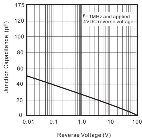
Fig.2 - Junction Capacitance
