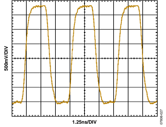
Figure 16. Typical Output Waveform, CMOS (250 MHz, 15 pF Load)
