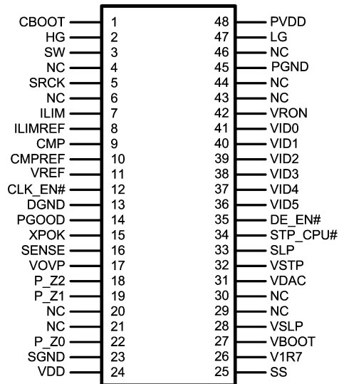
48-Lead TSSOP (MTD) See NS Package Number MTD48
