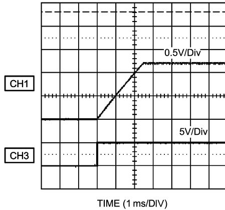
Turn-On Waveforms
