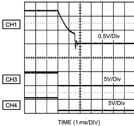
Turn-Off Waveforms
