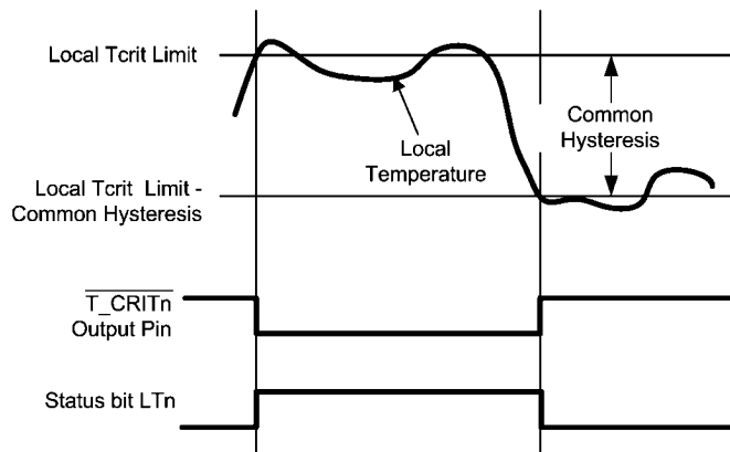
FIGURE 7. TCRIT response diagram (masking options not included)
