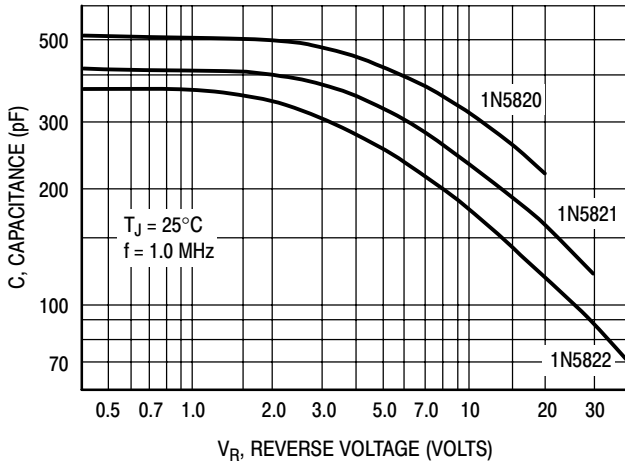
Figure 10. Typical Capacitance
