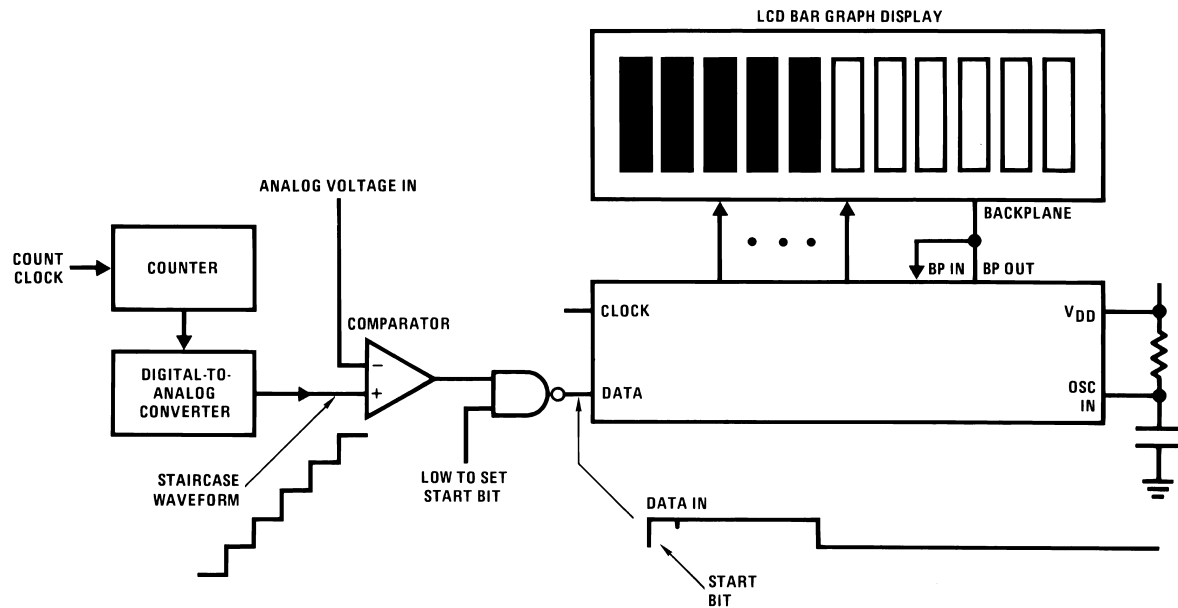
FIGURE 9. Four Wire Remote Display
