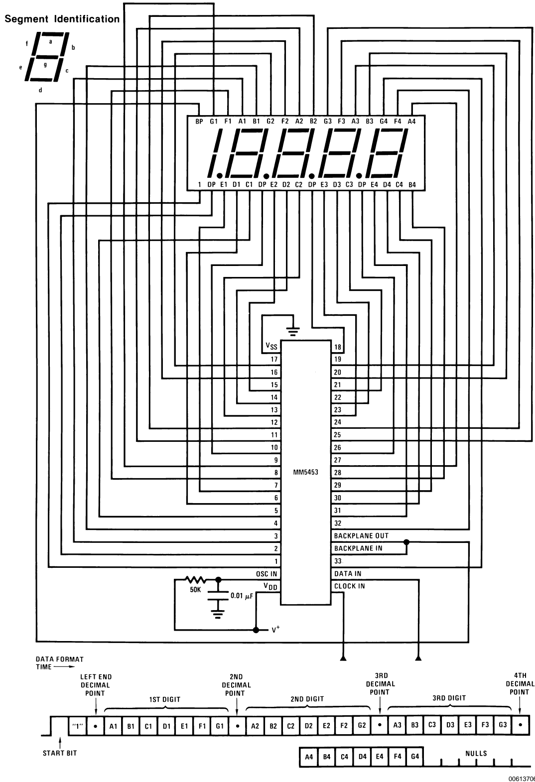
FIGURE 6. Typical 4½-Digit Display Application
