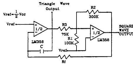
FIGURE 1 - FUNCTION GENERATOR
