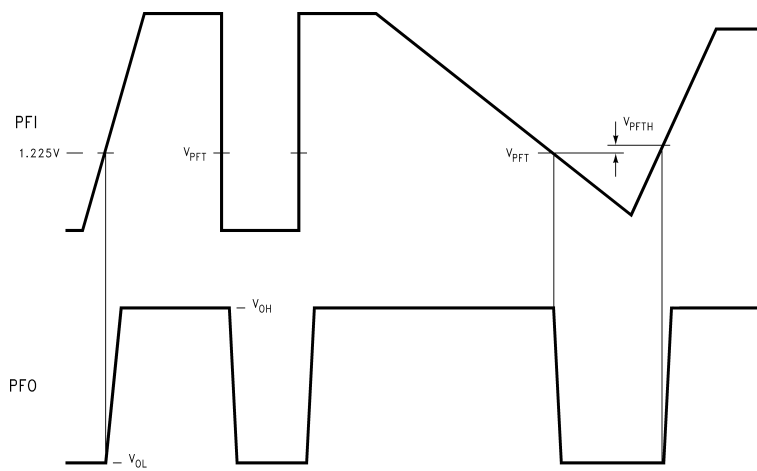
FIGURE 3. PFI Comparator Timing Diagram
