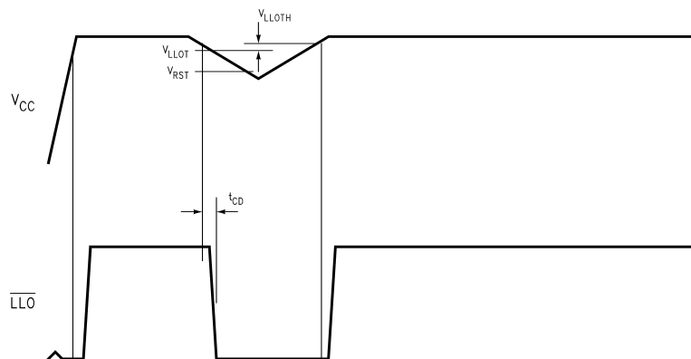
FIGURE 2. \overline{LLO} Output
