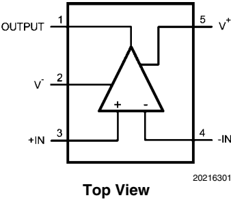
5-Pin SOT-23 (LMV793)
