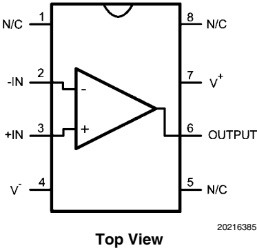
8-Pin SOIC (LMV793)
