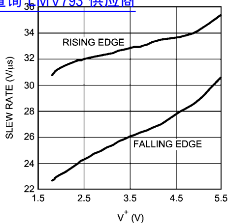
查询"LMV793"供应商 Slew Rate vs. Supply Voltage
