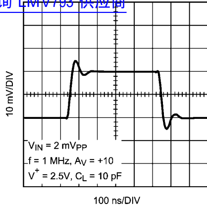
Small Signal Transient Response, A_V = +10 查询"LMV793"供应商
