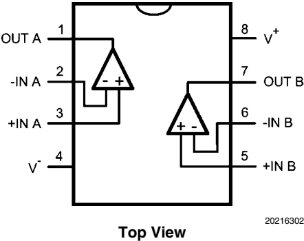
8-Pin SOIC/MSOP (LMV794)
