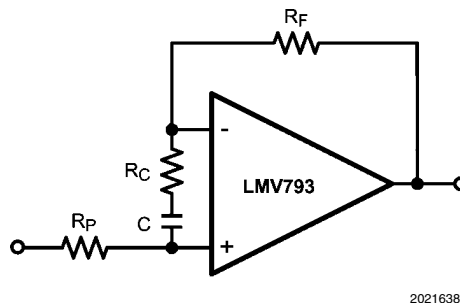
FIGURE 13. LMV793 with Lead-Lag Compensation for Non-Inverting Configuration
