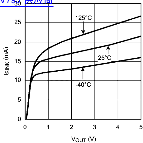
查询"LMV793"供应商 Sinking Current vs. Output Voltage
