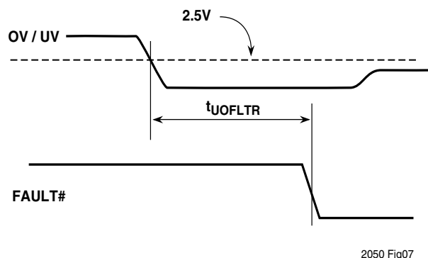
Figure 3. Under-/Over-Voltage Filter Timing
