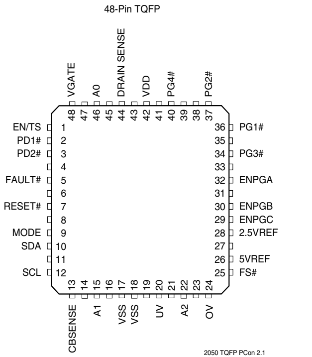
Figure 11. 48-Pin TQFP Package Pinout 1
