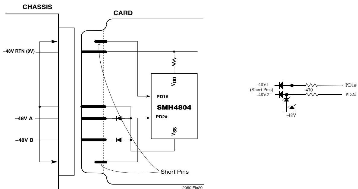
Figure 19. PD1# and PD2# Inputs, Physical Offset
