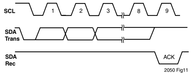
Figure 21. Acknowledge Timing
