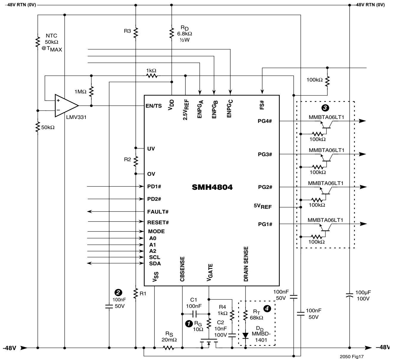
Figure 16. Over-temperature Shutdown
