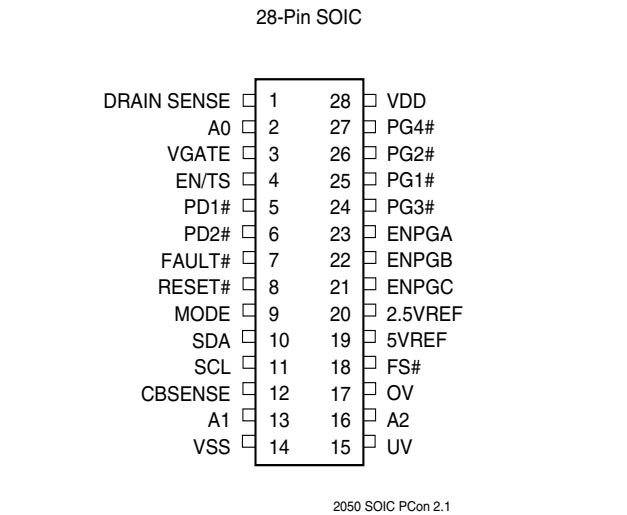
Figure 10. 28-Pin SOIC Package Pinout
