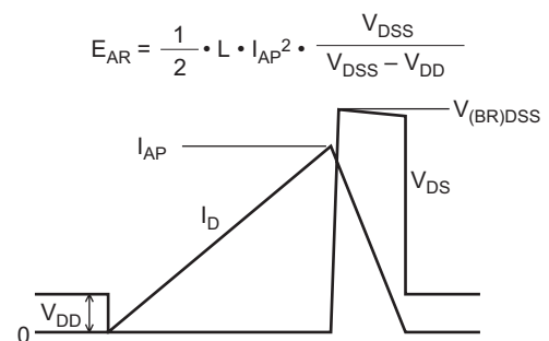
Avalanche Waveform
