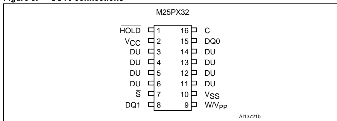
Figure 3. SO16 connections
