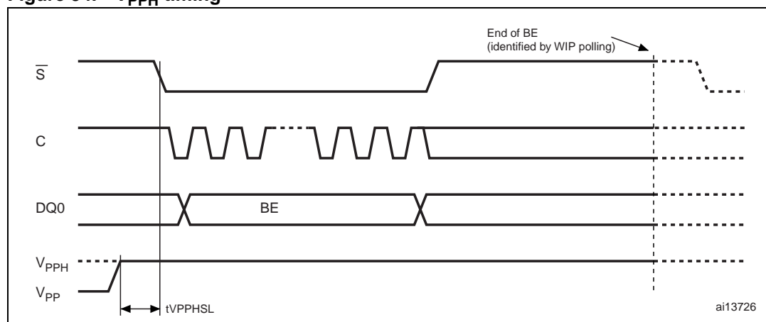
Figure 34. V_{PPH} timing
