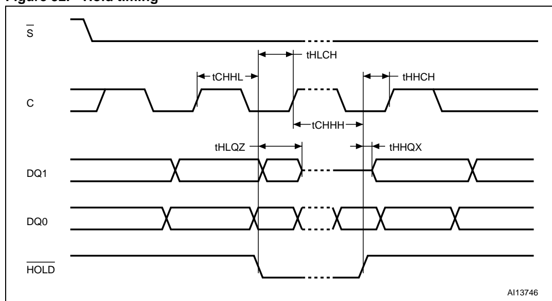
Figure 32. Hold timing
