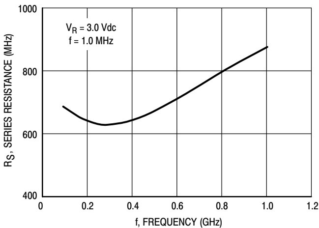
Figure 3. Series Resistance
