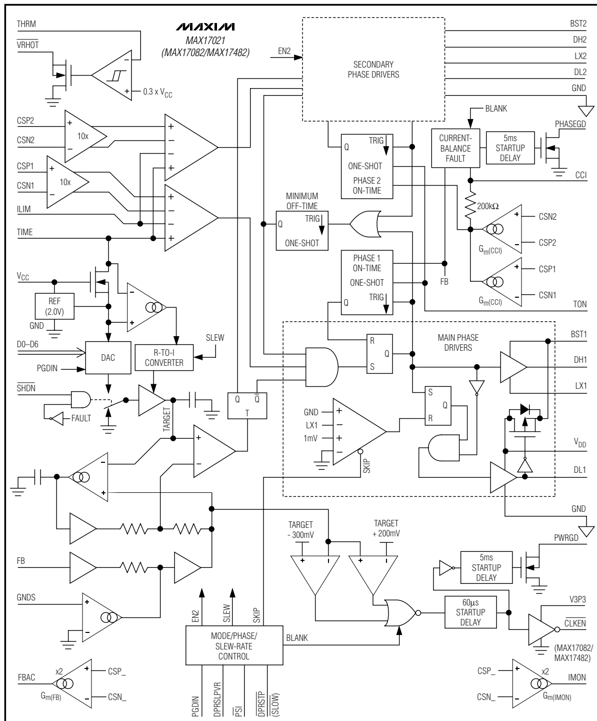
Figure 3. Functional Diagram
