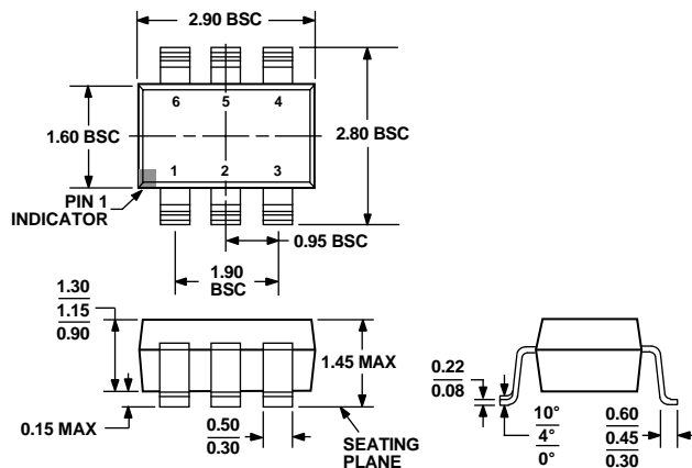
Figure 20. 6-Lead Small Outline Transistor Package [SOT-23] (RT-6)
