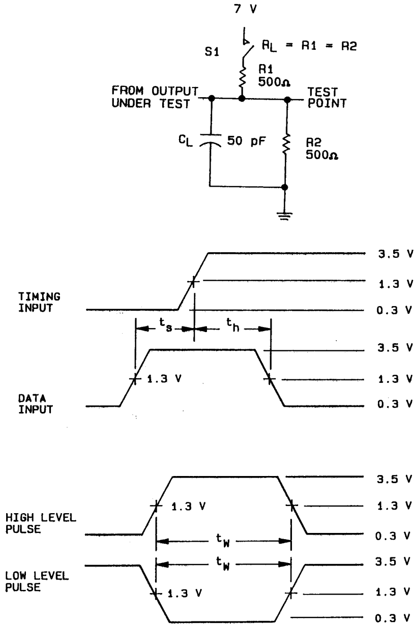
FIGURE 3. Test circuit and switching waveforms.
