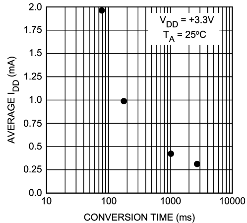
FIGURE 1. Conversion Rate Effect on Power Supply Current
