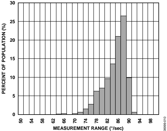
Figure 10. Measurement Range
