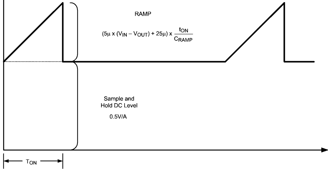
FIGURE 6. Composition of Current Sense Signal
