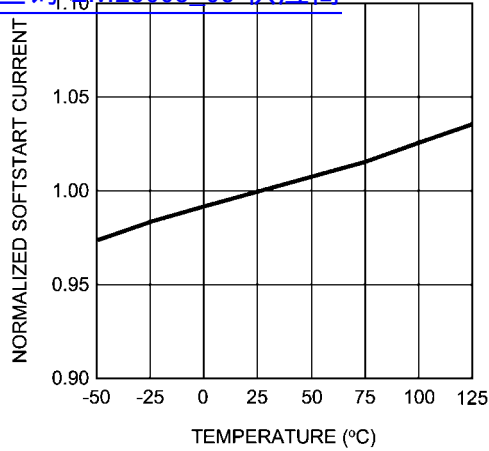
Soft Start Current vs Temperature 查询"LM25005_06"供应商
