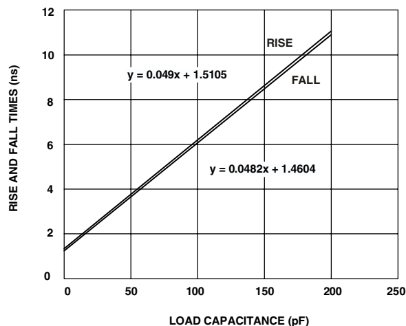
Figure 41. Typical Output Rise/Fall Time (20% to 80%, V DDEXT = Min)
