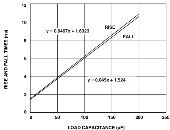
Figure 40. Typical Output Rise/Fall Time (20% to 80%, V DDEXT = Max)
