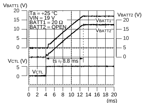
Soft-start operation waveform voltage mode (Li4C42)
