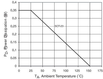
Power Derating
