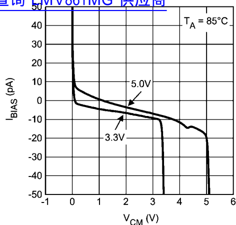
Input Bias Current vs. V_{CM} at 85°C 查询"LMV861MG"供应商
