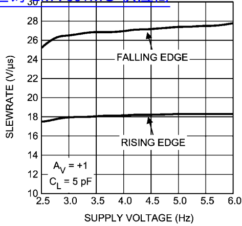
Slew Rate vs. Supply Voltage 查询"LMV861MG"供应商
