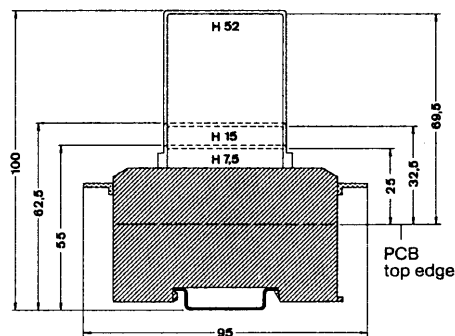
Dimensional drawing of electronic module EMG
