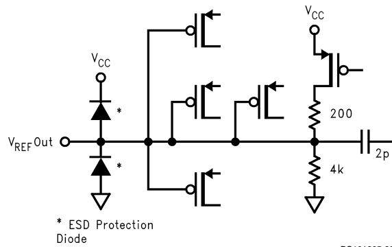
FIGURE 22. Pin 26 V_{REF} Out
