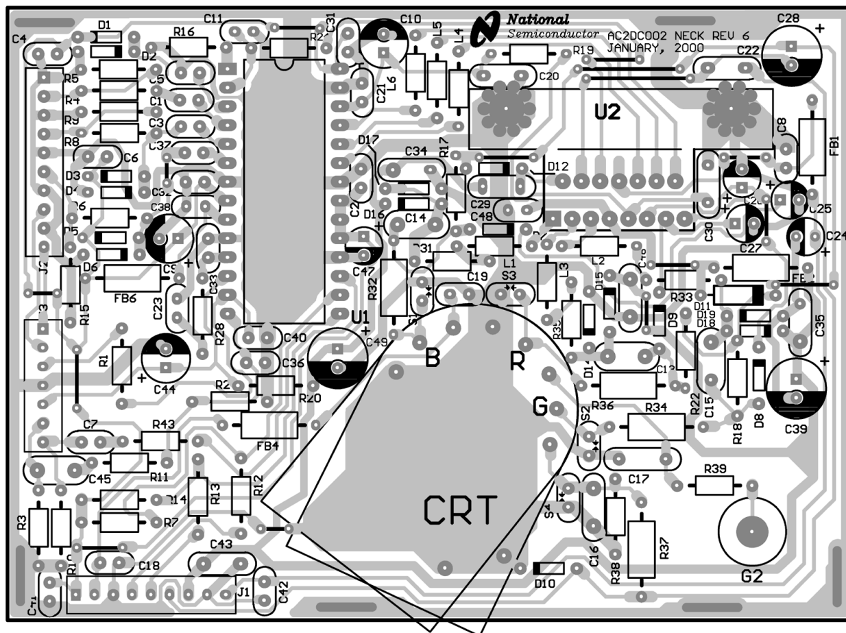
FIGURE 31. LM1253A/LM2453 Demo Board Layout
