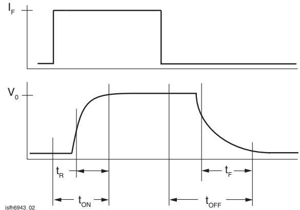
Figure 2. Switching Waveform
