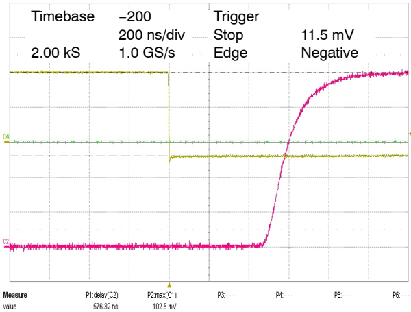
Figure 14. 20 mV Overdrive
