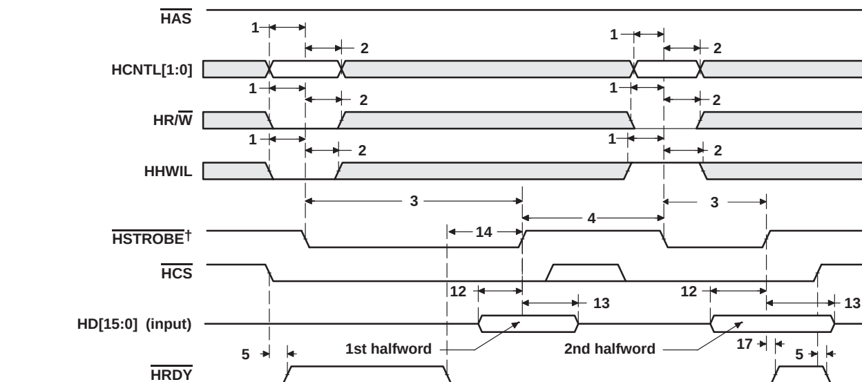
Figure 48. HPI Write Timing (HAS Not Used, Tied High)
