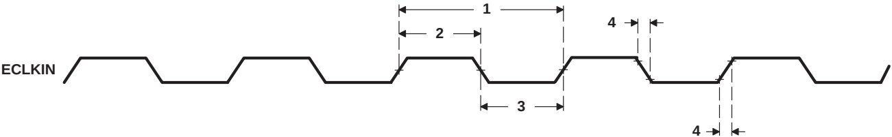
Figure 28. ECLKIN Timings
