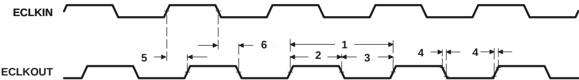
Figure 29. ECLKOUT Timings
