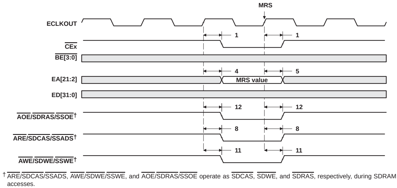
Figure 40. SDRAM MRS Command
