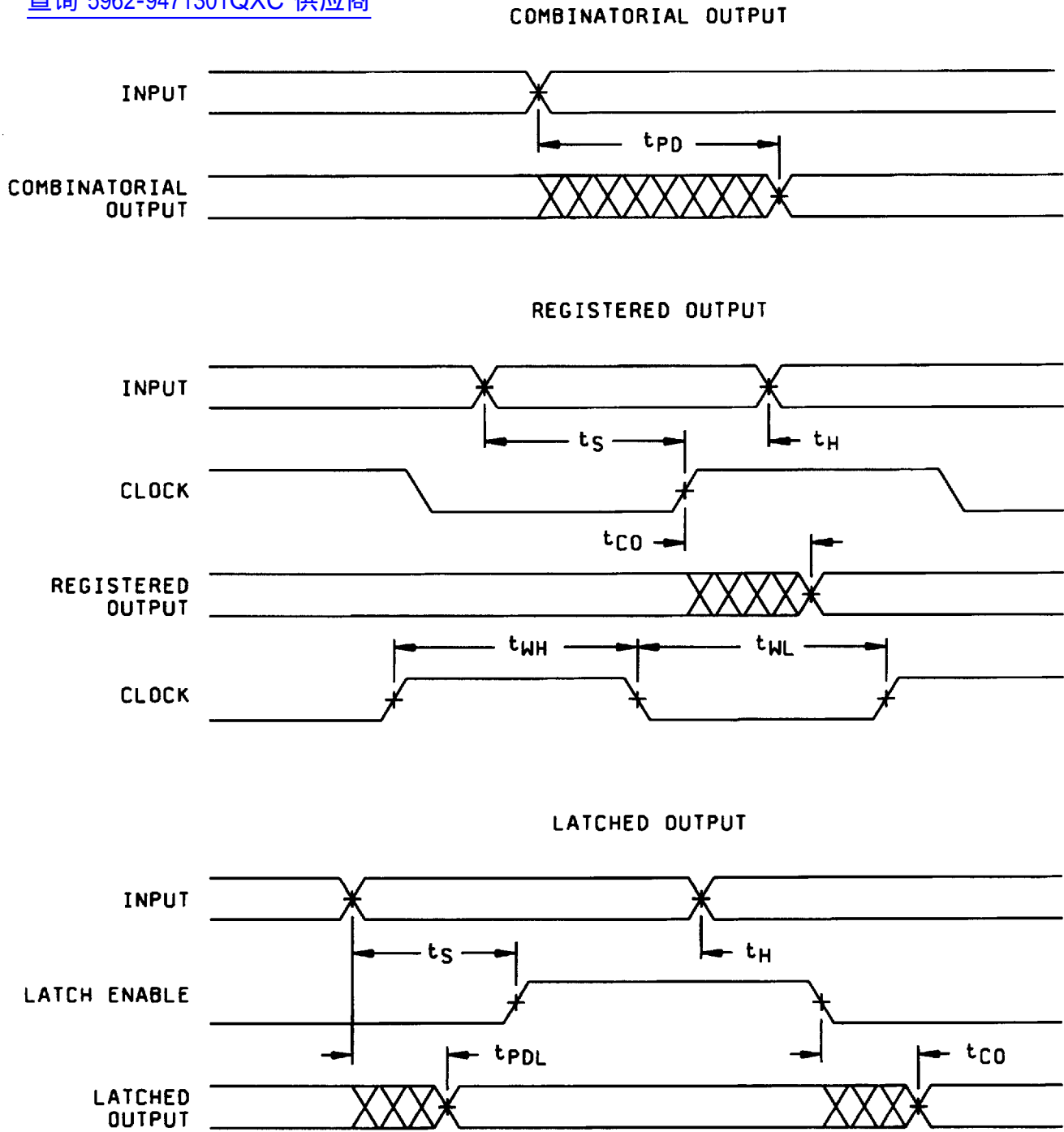
FIGURE 4. Switching waveforms.
