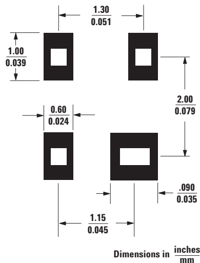
Figure 12. Recommended PCB Pad Layout for Agilent's SC70 4L/SOT-343 Products.
