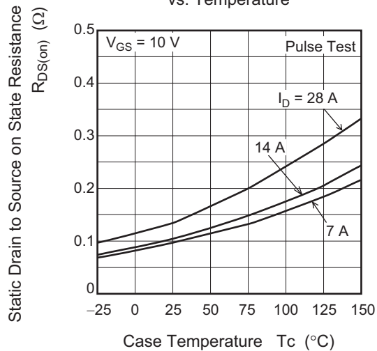
Static Drain to Source Resistance vs. Temperature
