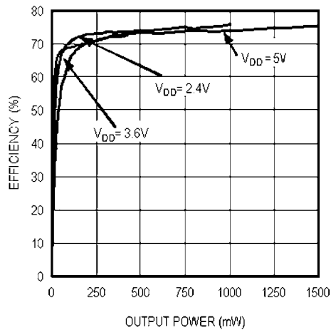
Efficiency vs Output Power R_L = 15\mu H + 4\Omega + 15\mu H , f = 1\text{kHz}, 22\text{kHz BW}
