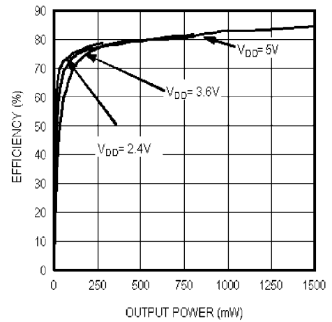
Efficiency vs Output Power R_L = 15\mu H + 8\Omega + 15\mu H , f = 1\text{kHz}, 22\text{kHz BW}
