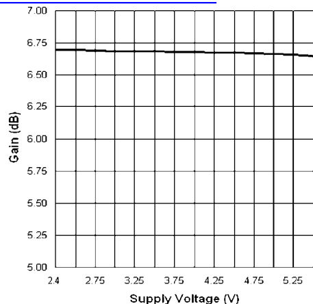
Gain vs Supply Voltage 查询"LM4671" (5500) R_L = 15\mu H
