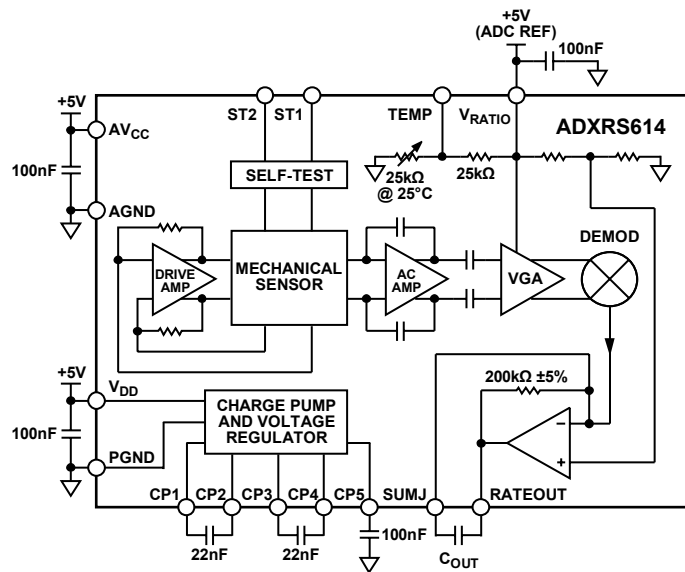
Figure 1. ADXR5614 Block Diagram
